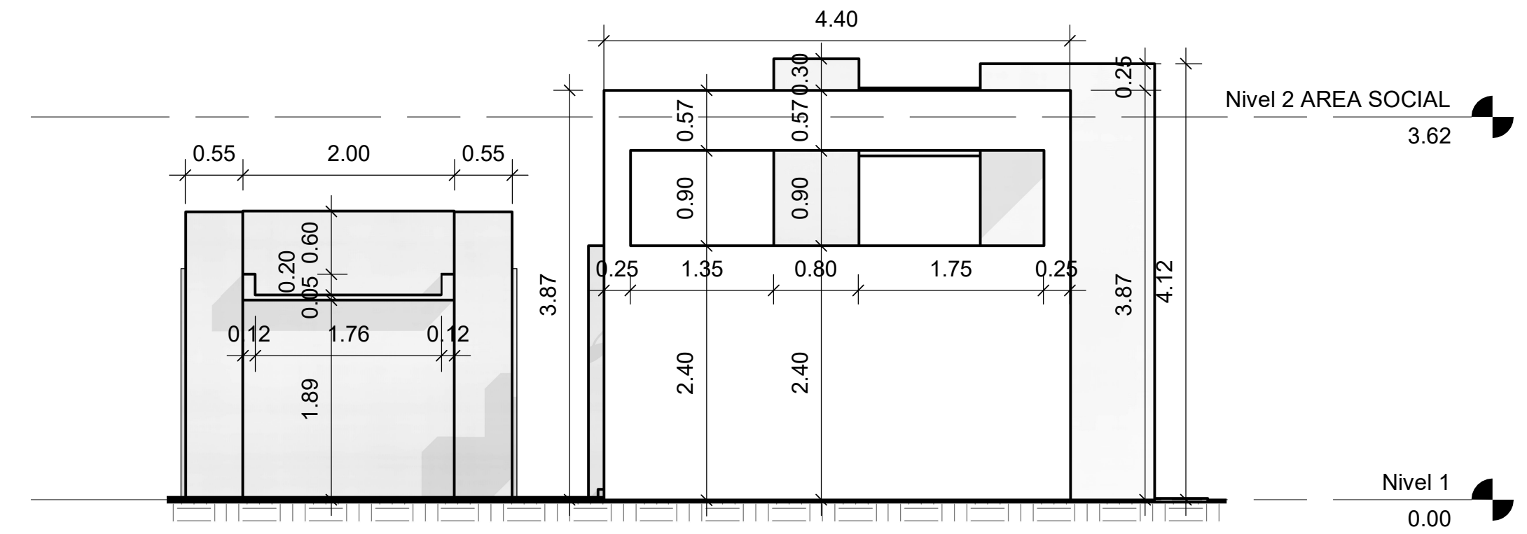
BAVARO ISLAND RESIDENCES 2 ELEVACION V2 AREA SOCIAL Residencial Bavaro Island 1 : 50
