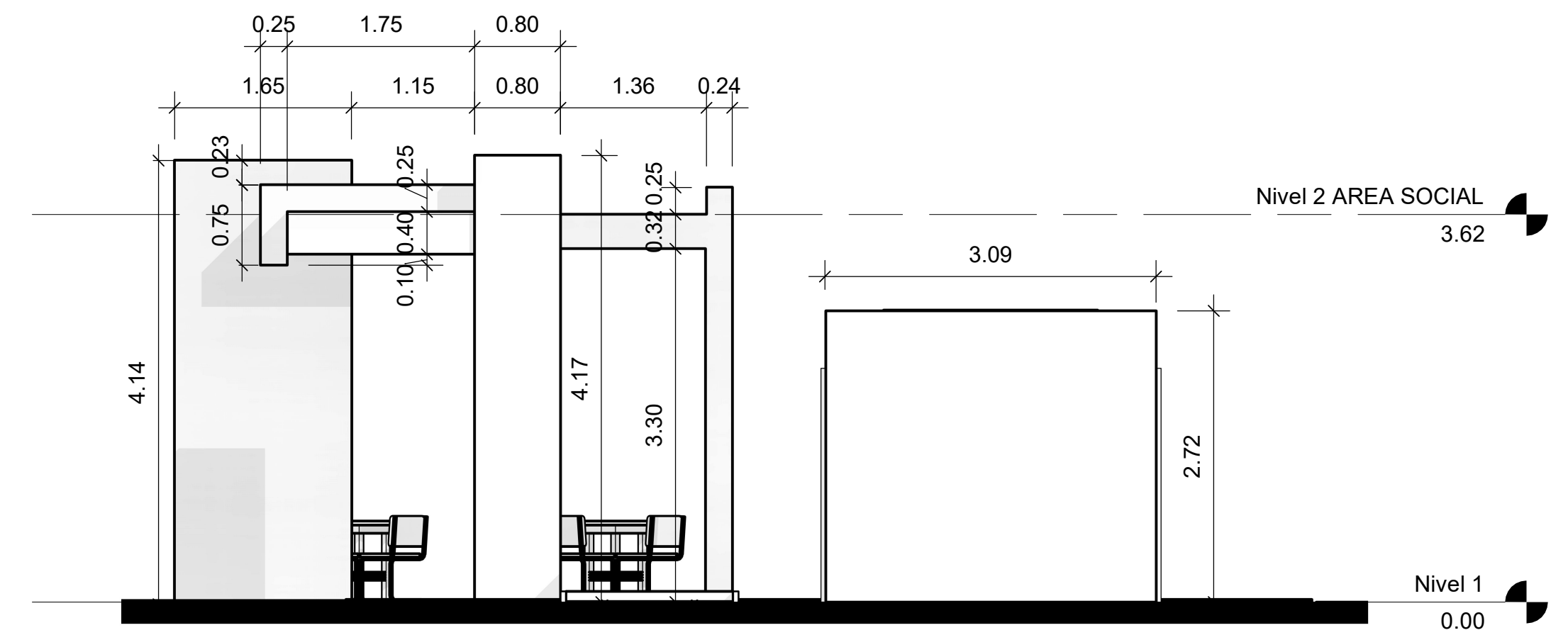
BAVARO ISLAND RESIDENCES 4 ELEVACION V4 AREA SOCIAL Residencial Bavaro Island 1 : 50
