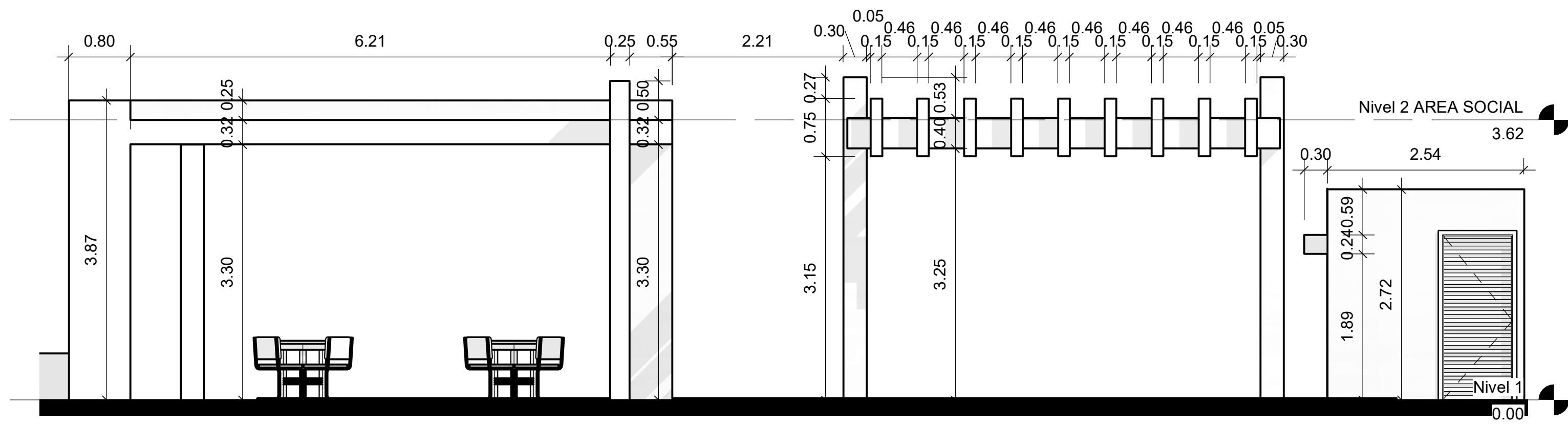
BAVARO ISLAND RESIDENCES 1.1 ELEVACION V1 AREA SOCIAL Residencial Bavaro Island 1 : 50
