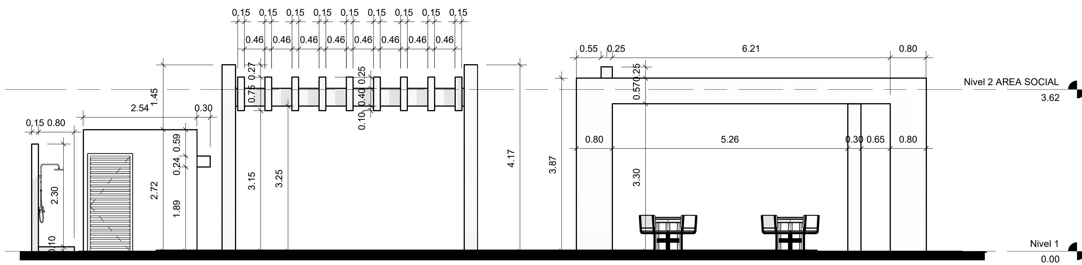
BAVARO ISLAND RESIDENCES 3 ELEVACION V3 AREA SOCIAL Residencial Bavaro Island 1 : 50
